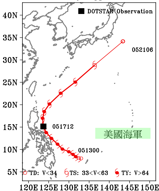
JTWC Best Track of Typhoon Nida(2004)
